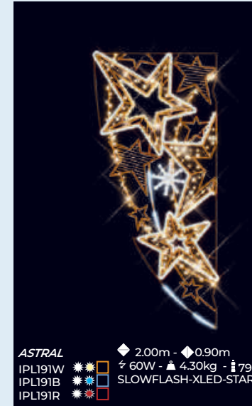
ASTRAL IPL191R * * * □ IPL191W * * * □ IPL191B * * * □ ◆ 2.00m - ◆ 0.90m ⚡ 60W - ⚠ 4.30kg - ⚡ 79 SLOWFLASH-XLED-STARS
